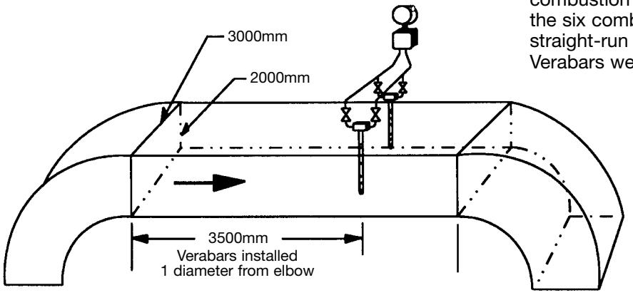
Figure 1 Installation for duct air flow in Huang Pu Power Plant
