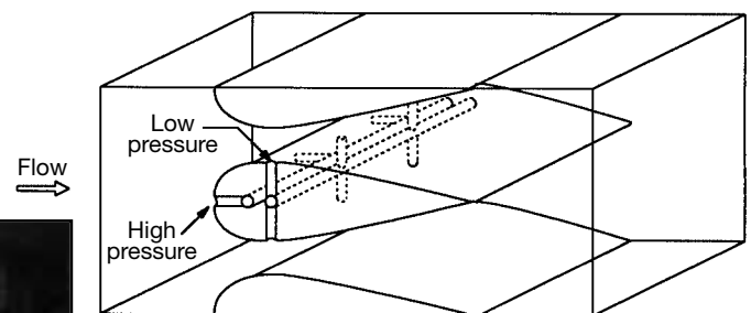
Figure 2 Old airfoils
